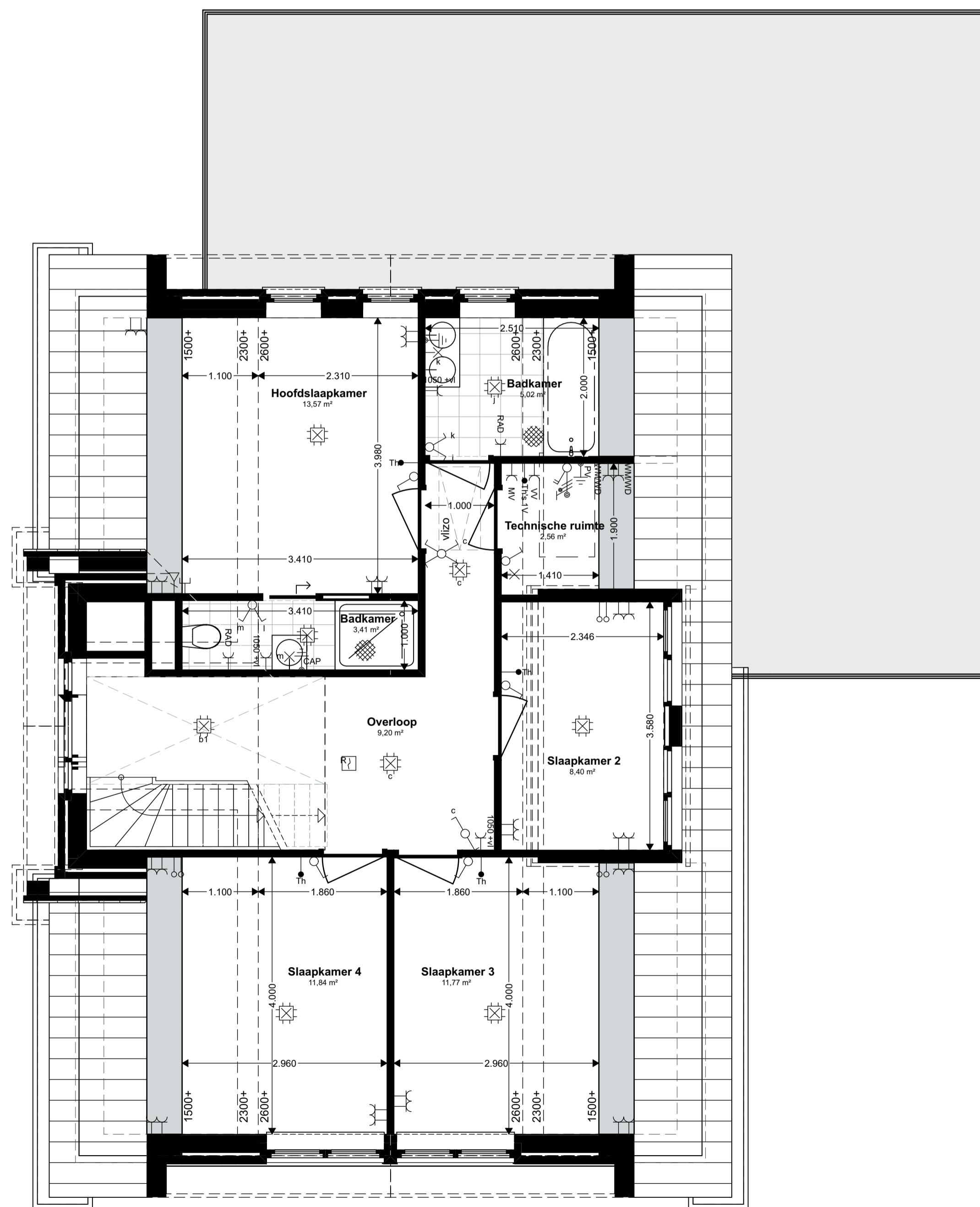
Verdieping (1:50)
