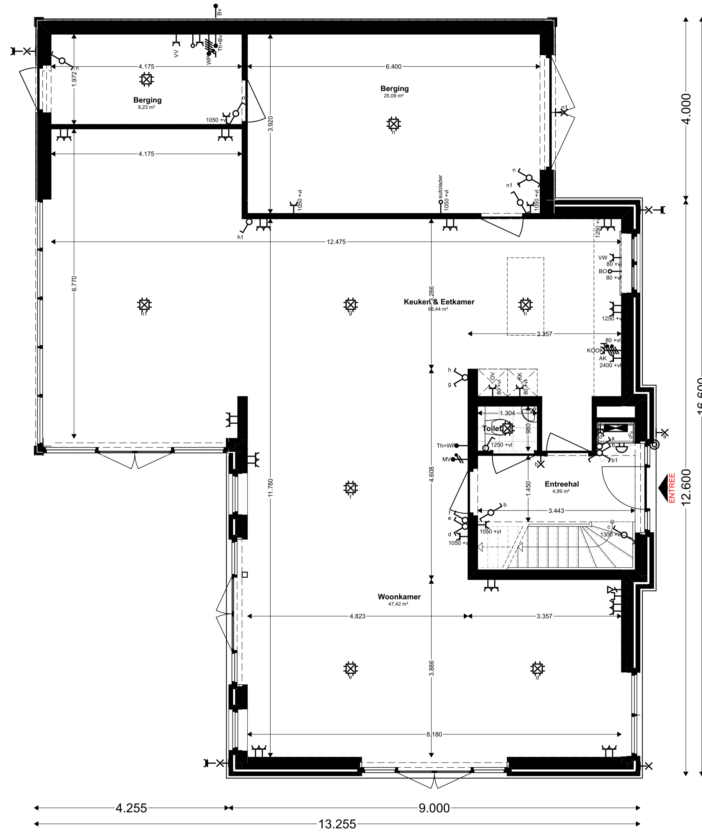
Begane grond (1:50)
