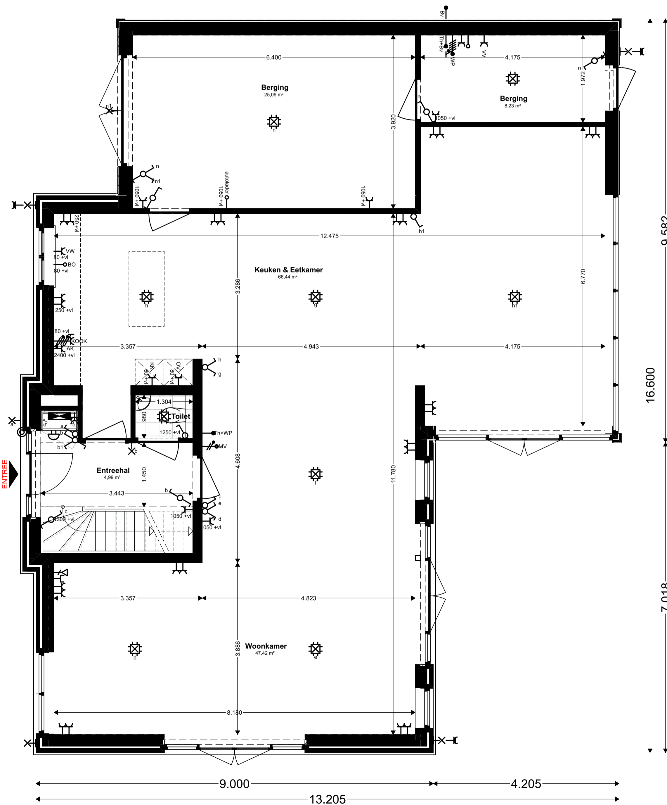
Begane grond (1:50)
