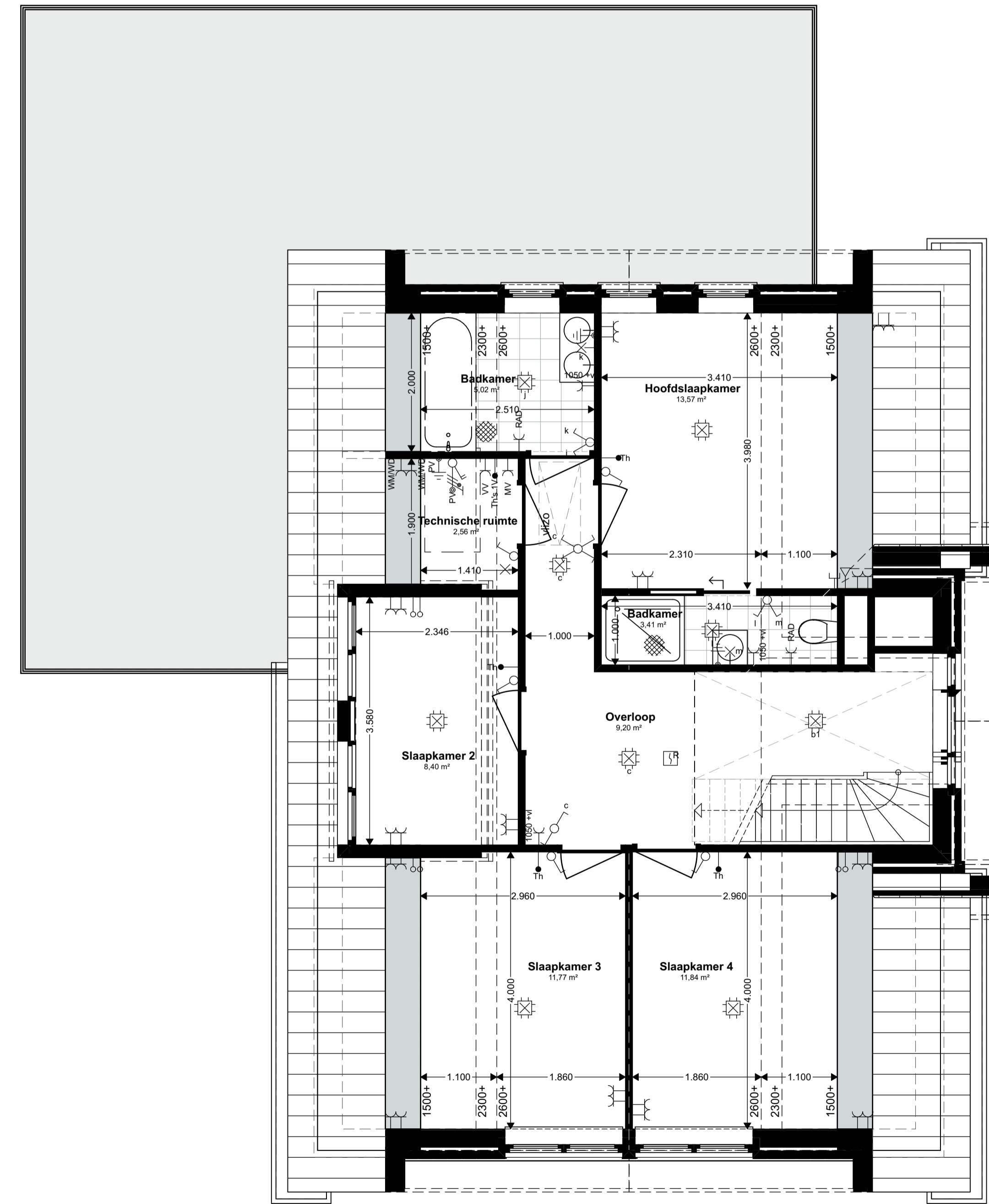
Verdieping (1:50)
